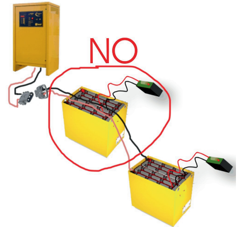
fig.2 incorrect position of the cables.
